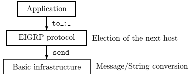
Figure 2. Layers for distributed applications
